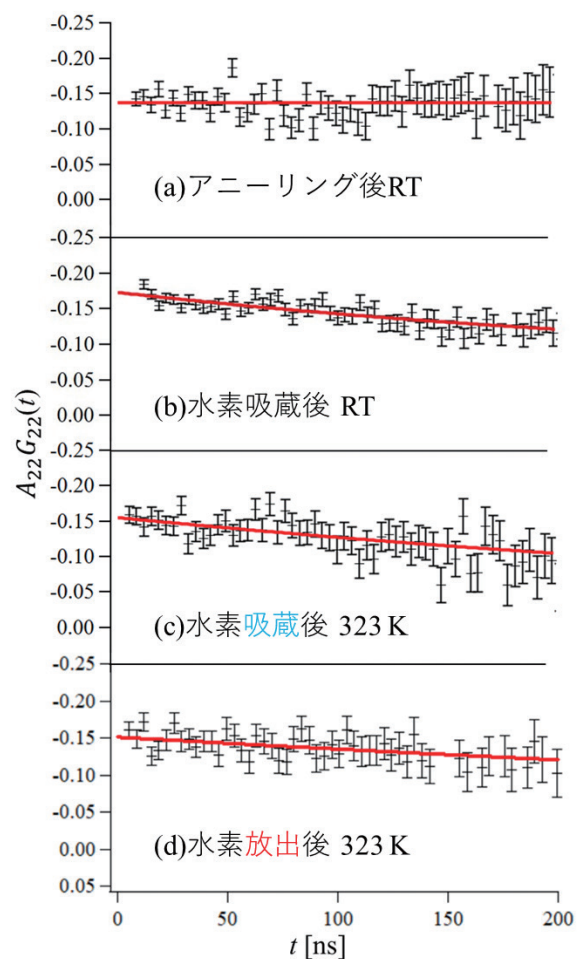
Fig. 1 PAC spectra of the ^{111}\text{Cd} ( \leftarrow ^{111}\text{Ag} \leftarrow ^{111,111\text{m}}\text{Pd} ) probe in a hydrogen-absorbed Pd plate.
